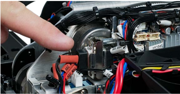
5. Locate the 9-pin connector and carefully unplug it from its socket. DO NOT USE FORCE TO REMOVE!
