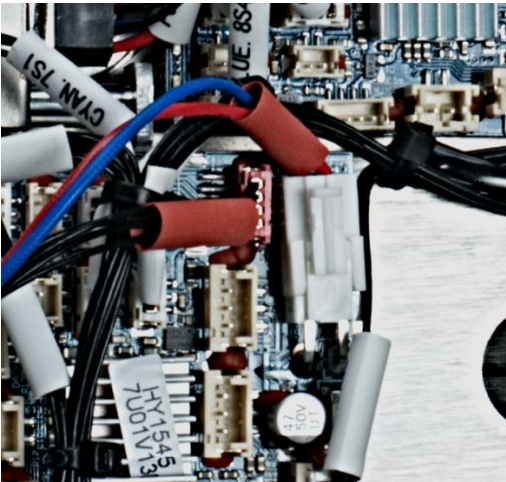
7. Unplug the 2-pin and 4-pin connectors that are attached to the module.
