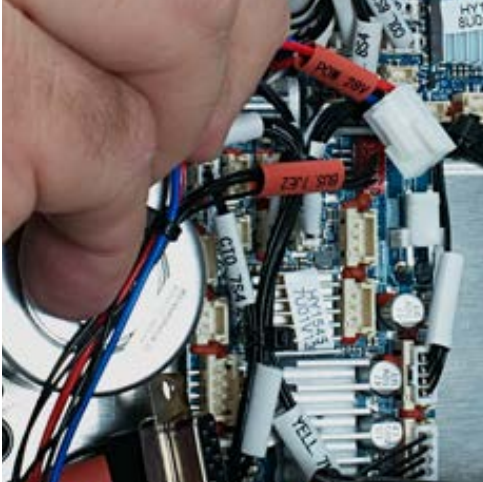
7. Unplug the 2-pin and 4-pin connectors that are attached to the module.
