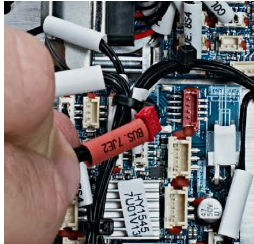
6. Carefully grip the GOBO Wheel module and slid it out just enough to reveal two more wire connectors.
