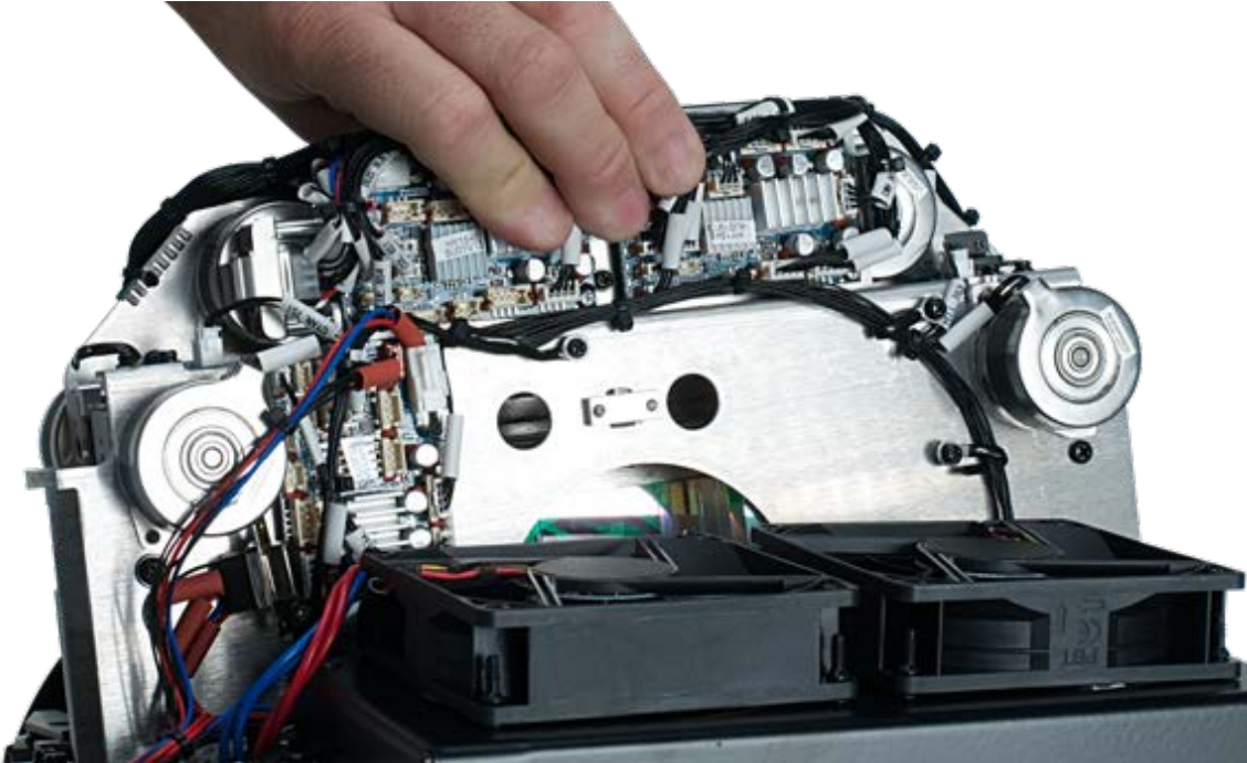
6. Carefully grip the GOBO Wheel module and slid it out just enough to reveal two more wire connectors.
